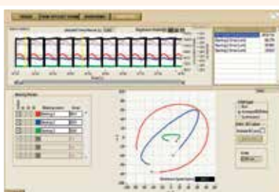
Orbit plot
